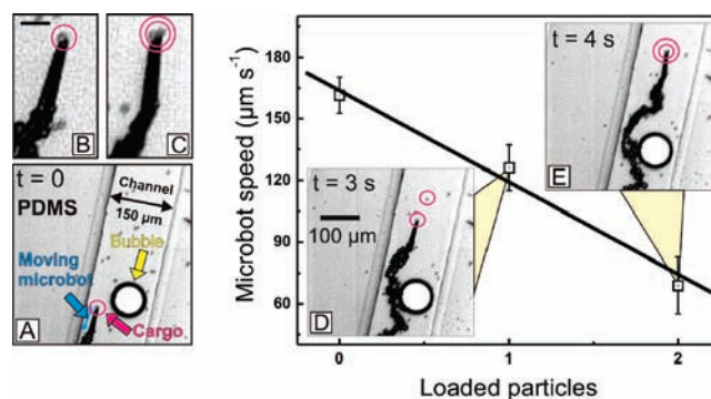
Figure 3. Catalytic Ti/Fe/Pt microbot loading and transporting 5 \mu\text{m} diameter polystyrene particles into microfluidic channels. The plot shows the dependence of the microbot speed on the number of particles loaded. (A) Moving microbot sorting a residual bubble into a 150 \mu\text{m} wide microchannel in a PDMS microchip. (B, C) Zoomed images of the microbot loading (B) one and (C) two microparticles. (D, E) Microbot transporting (D) one and (E) two microparticles into the microchannels.
